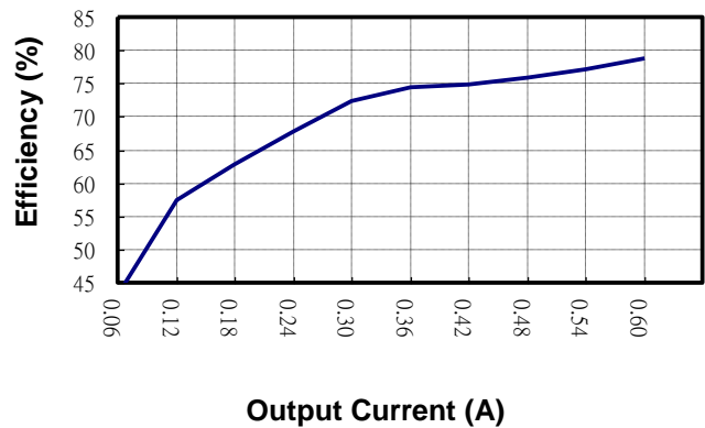
BOB3-48S1 Output Current vs. Efficiency
