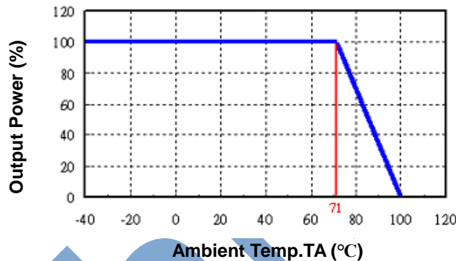
BOB3 Series Power Derating Curve(5)
