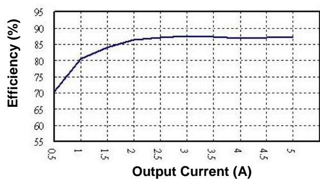
BVA25-48S1 Output Current vs. Efficiency
