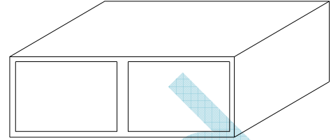
OUTER CARTON-598x287x150
